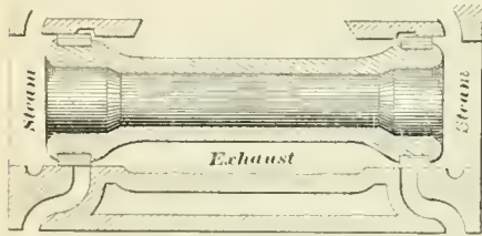
FIG. 6. LONG PISTON VALVE WITH OUTSIDE ADMISSION.
